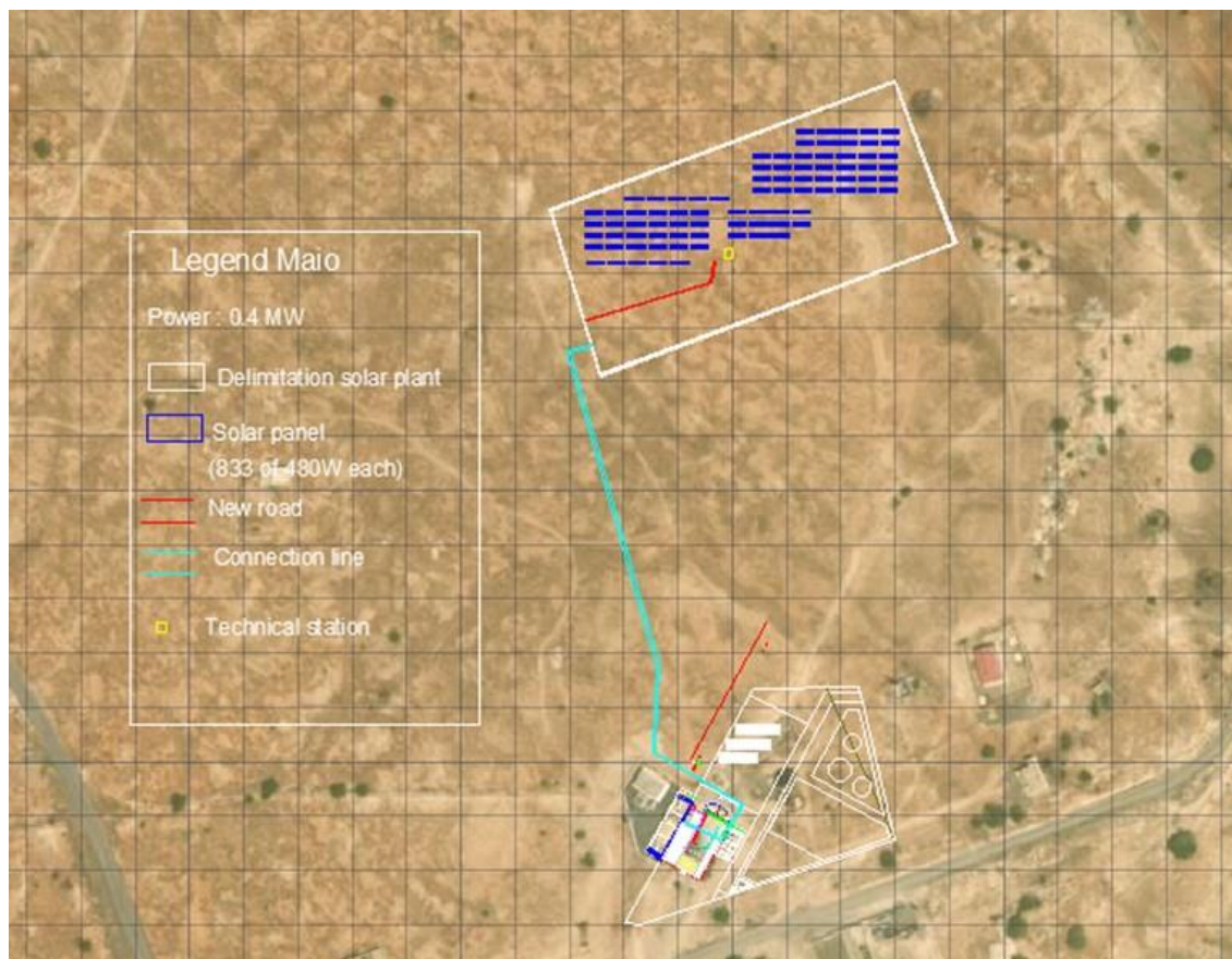
Figure 3 - Deployment of the solar PV plant on the plot of land
