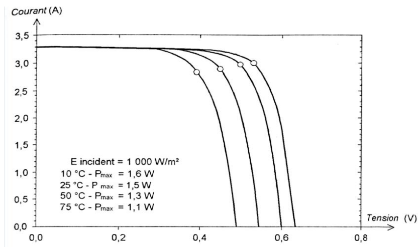
Figure 5 - I (V) curve of a single-crystalline cell at various temperatures
