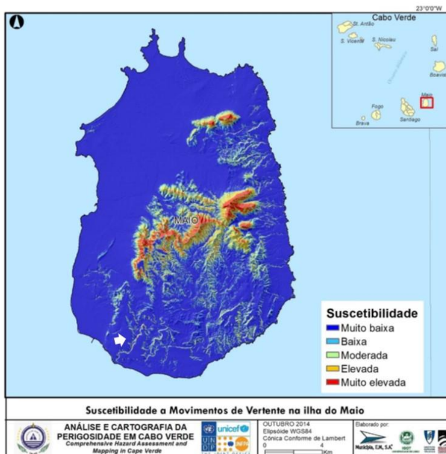
Figure 7 - Susceptibility to slope movement in Maio Island
