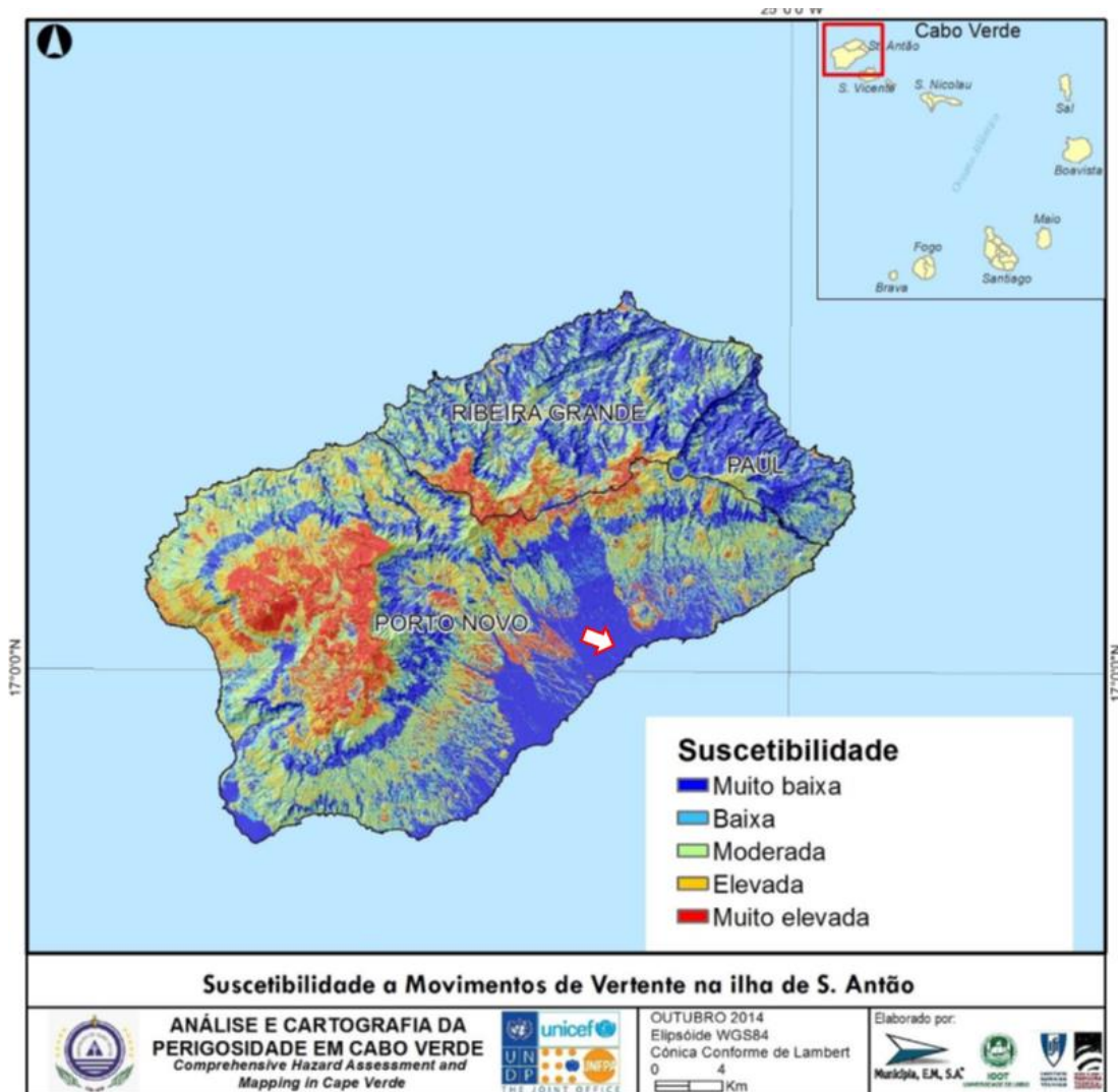
Figure 7 - Susceptibility to slope movement in Santo Antão Island
