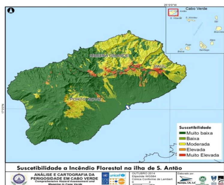
Figure 9 - Susceptibility to forest fire
